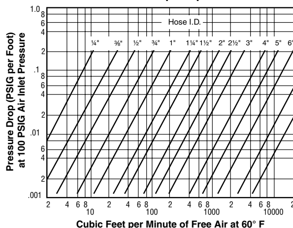
Pressure Drop Graph for Air
